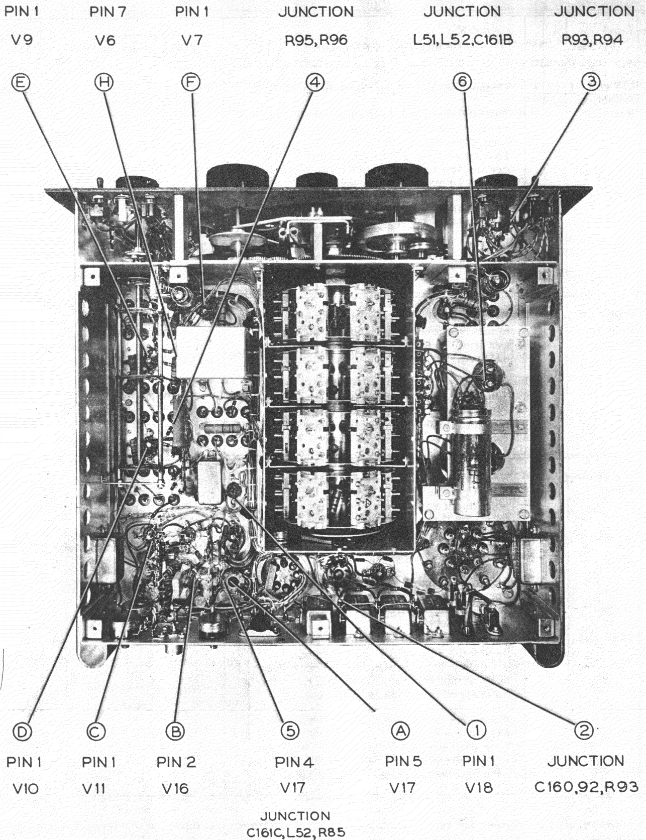
Figure 5-3. Radio Receiver Parts Identification for Locating Test Points
