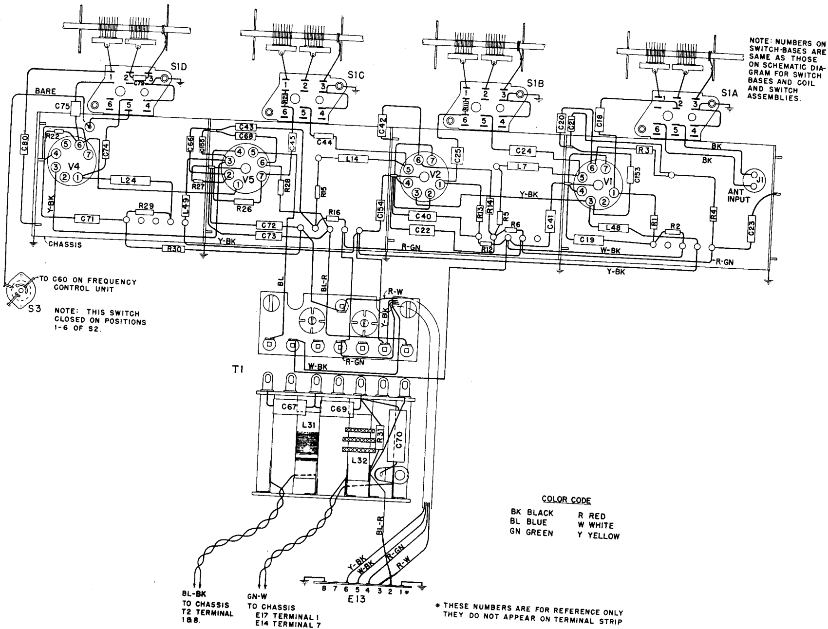
Figure 7-3. Radio Receiver, Tuning Unit Connection Diagram
