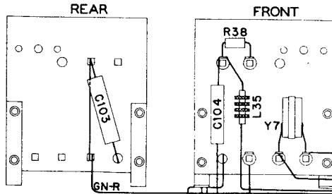
OSCILLATOR TERMINAL BOARD LOCATED OVER V8 & V6 SOCKETS ON BOTTOM OF CHASSIS. [SHIELDED]
